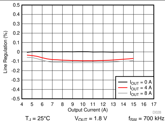
Figure 36. Line Regulation
