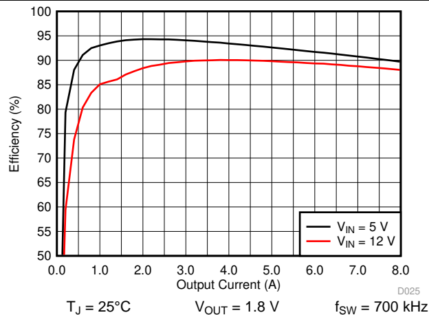
Figure 33. Efficiency
