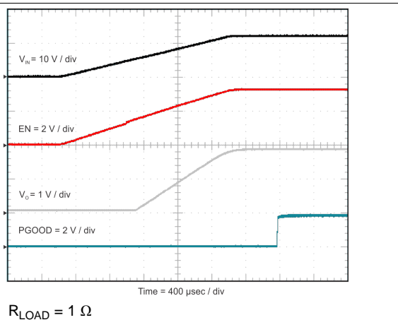
Figure 43. V_{IN} Startup
