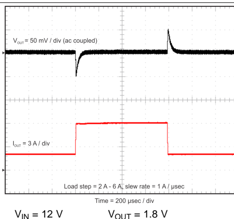
Figure 38. Transient Response
