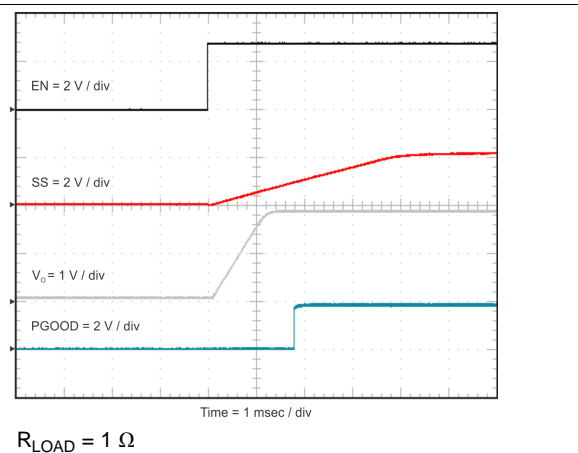
Figure 44. EN Startup
