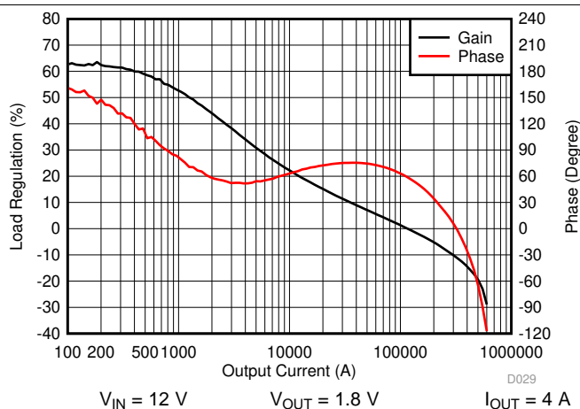
Figure 37. Loop Response
