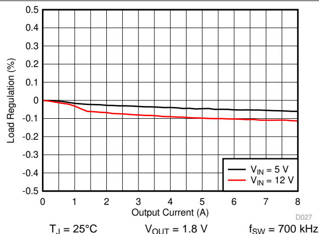
Figure 35. Load Regulation
