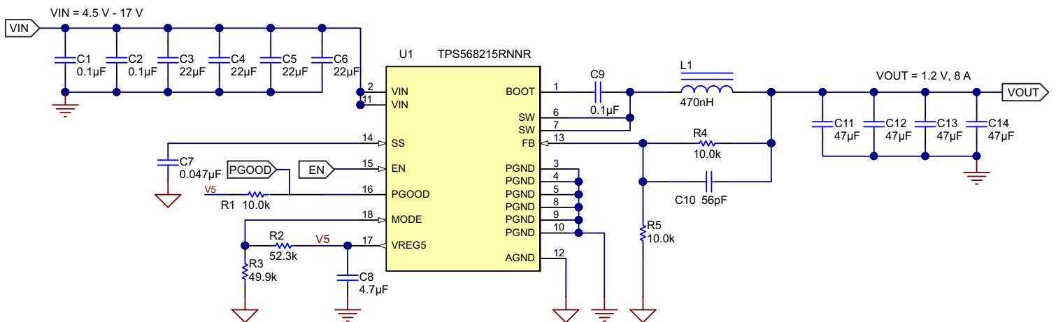
Figure 8-1. Application Schematic
