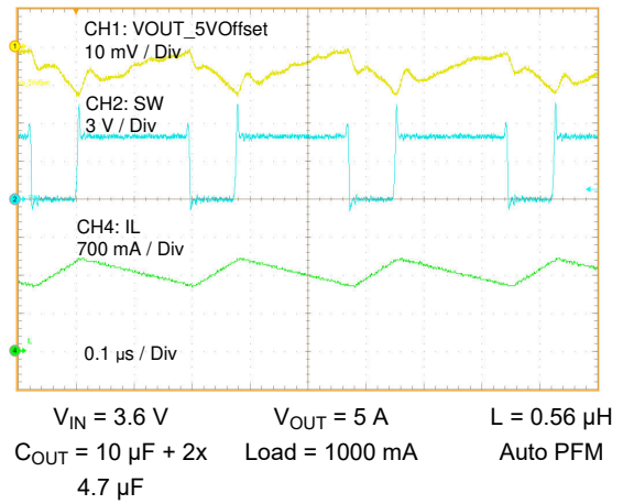
Figure 9-3. Steady 1000 mA
