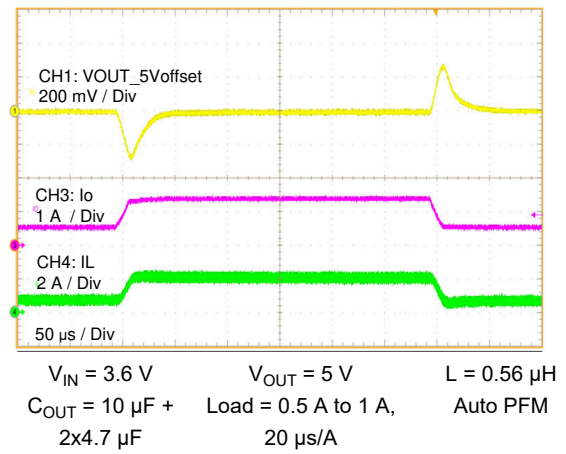
Figure 9-7. Load Transient
