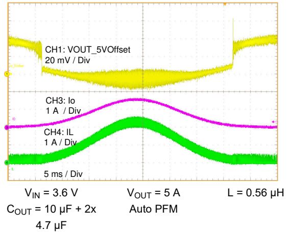
Figure 9-5. Load Sweep
