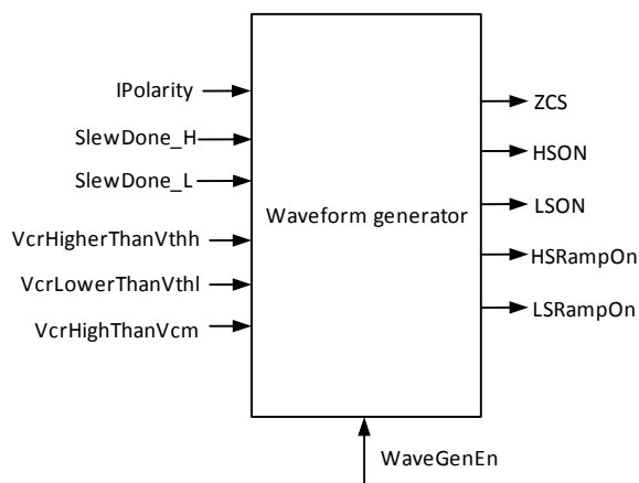
Figure 41. Waveform Generator State Machine Block Diagram
