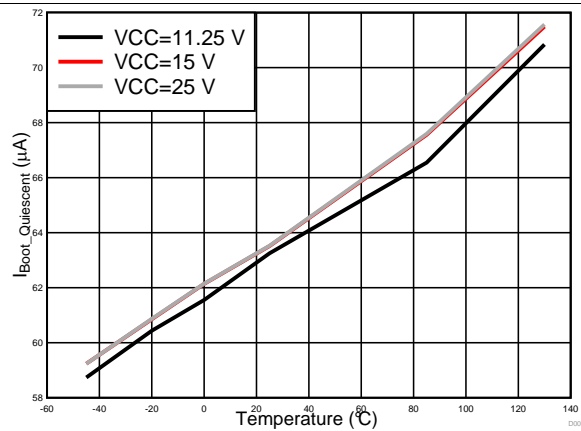
Figure 1. I BOOT_QUIESCENT vs Temperature
