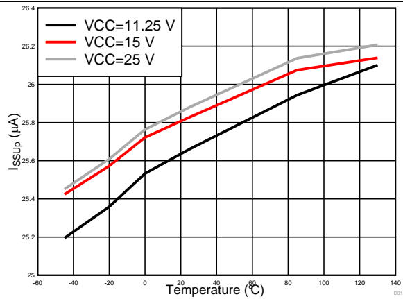
Figure 13. I_{SSUp} vs Temperature
