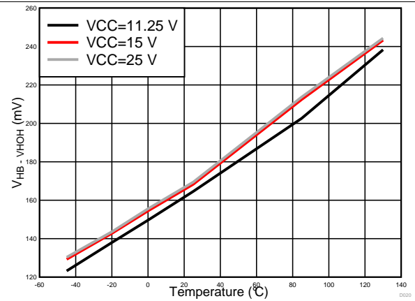
Figure 20. V_{HB} - V_{HOH} vs Temperature
