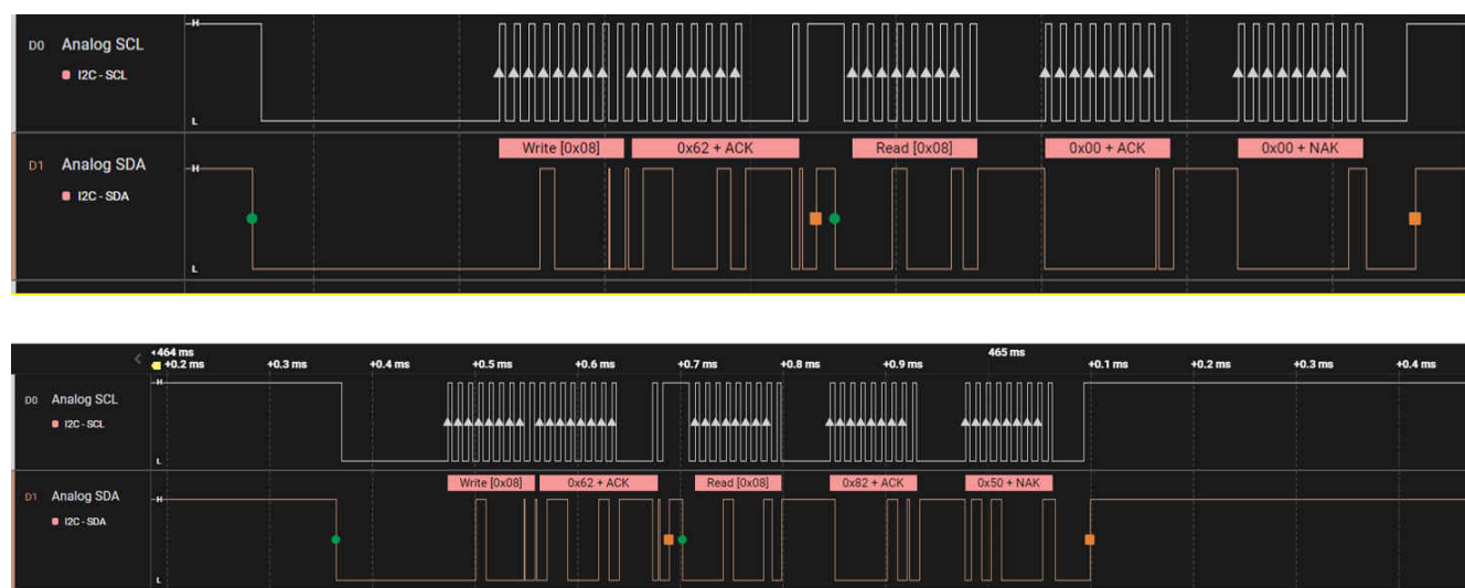
Figure 4-1. Captured I2C Waveform for Alarm Status Reading
