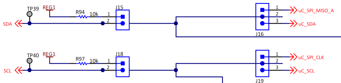
Figure 2-3. 3.3V Pullup for SDA and SCL on BQ76952EVM
