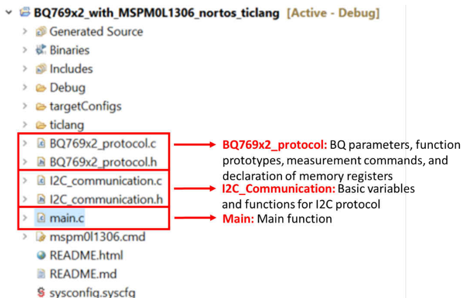
Figure 3-1. Software Project View
