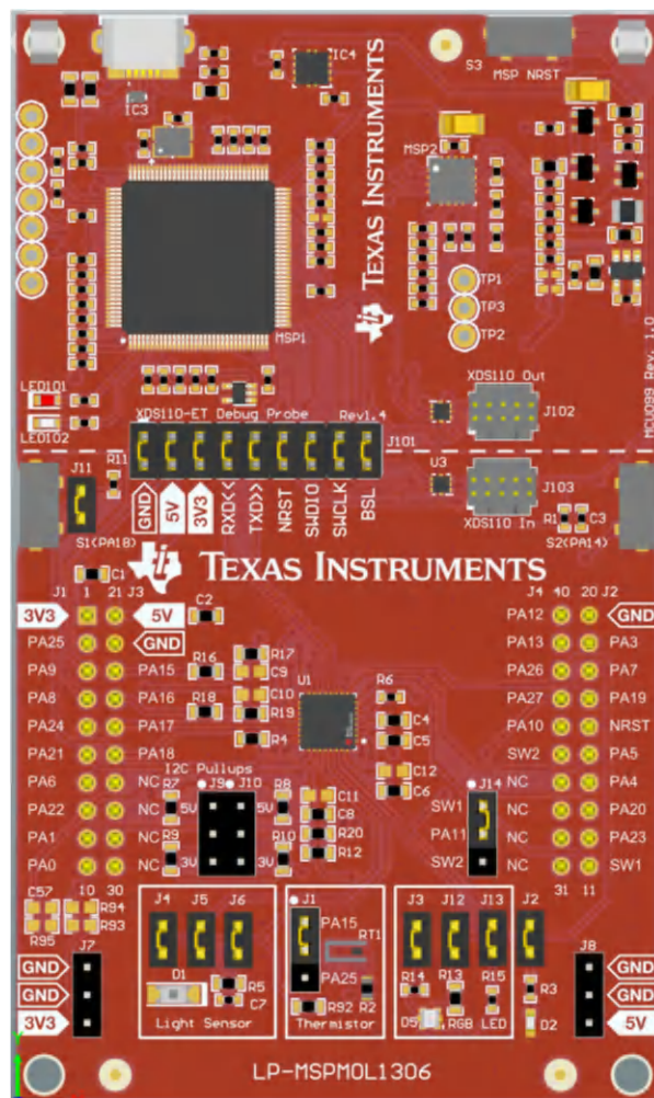
Figure 2-2. LP-MSPM0L1306 Hardware Board
